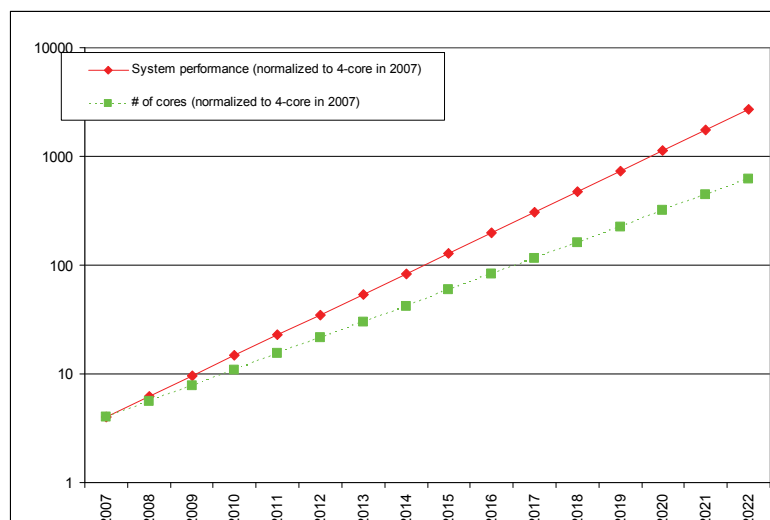
Figure SYSD2 SOC Networking Driver MC/AE Platform Performance
