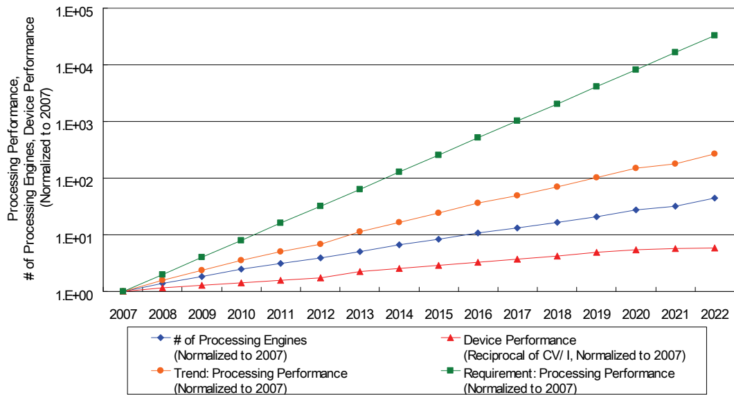
Figure SYSD7 SOC Consumer Portable Processing Performance Trends
