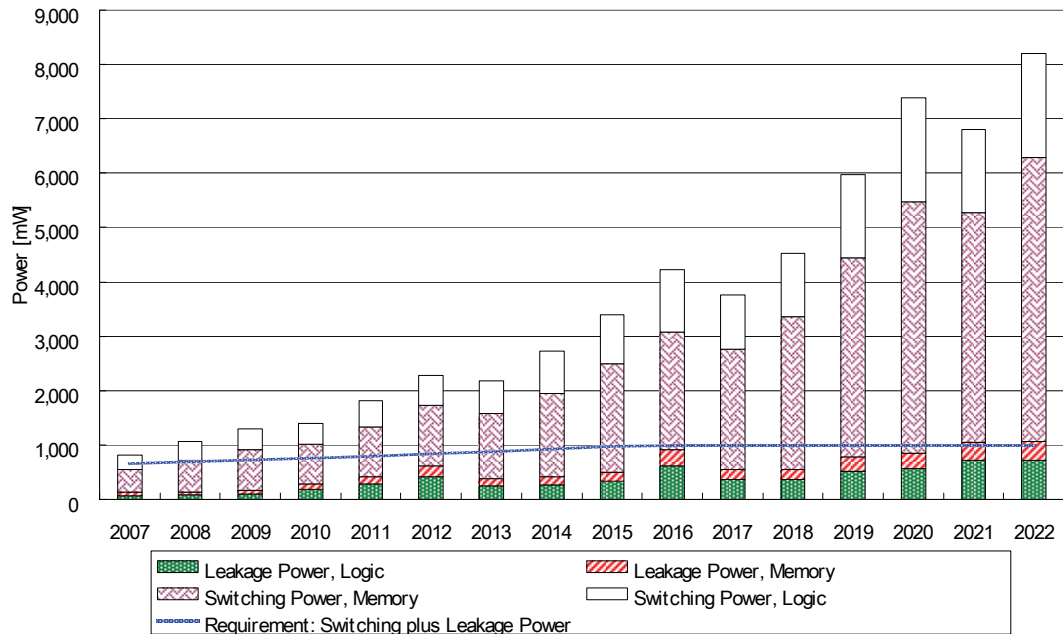
Figure SYSD6 SOC Consumer Portable Power Consumption Trends
