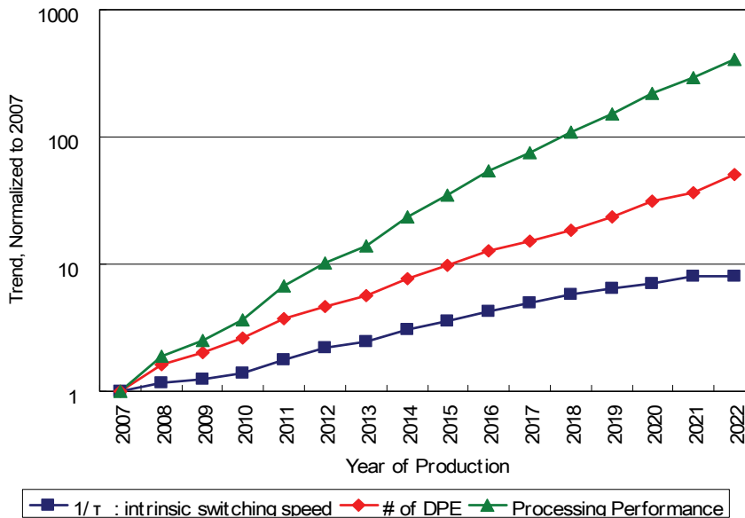
Figure SYSD10 SOC Consumer Stationary Performance Trends
