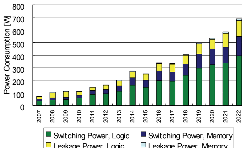
Figure SYS11 SOC Consumer Stationary Power Consumption Trends
