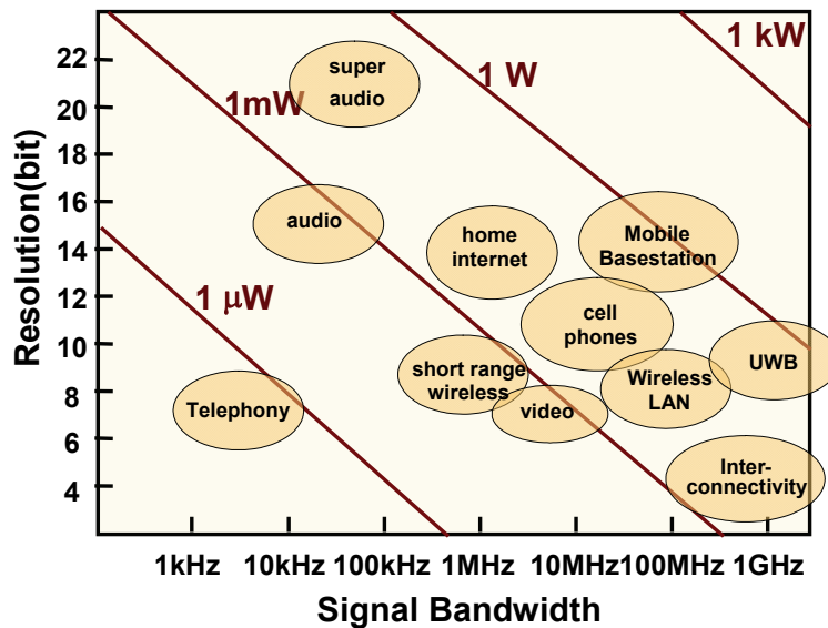
Figure SYSD12 Recent ADC Performance Needs for Important Product Classes
