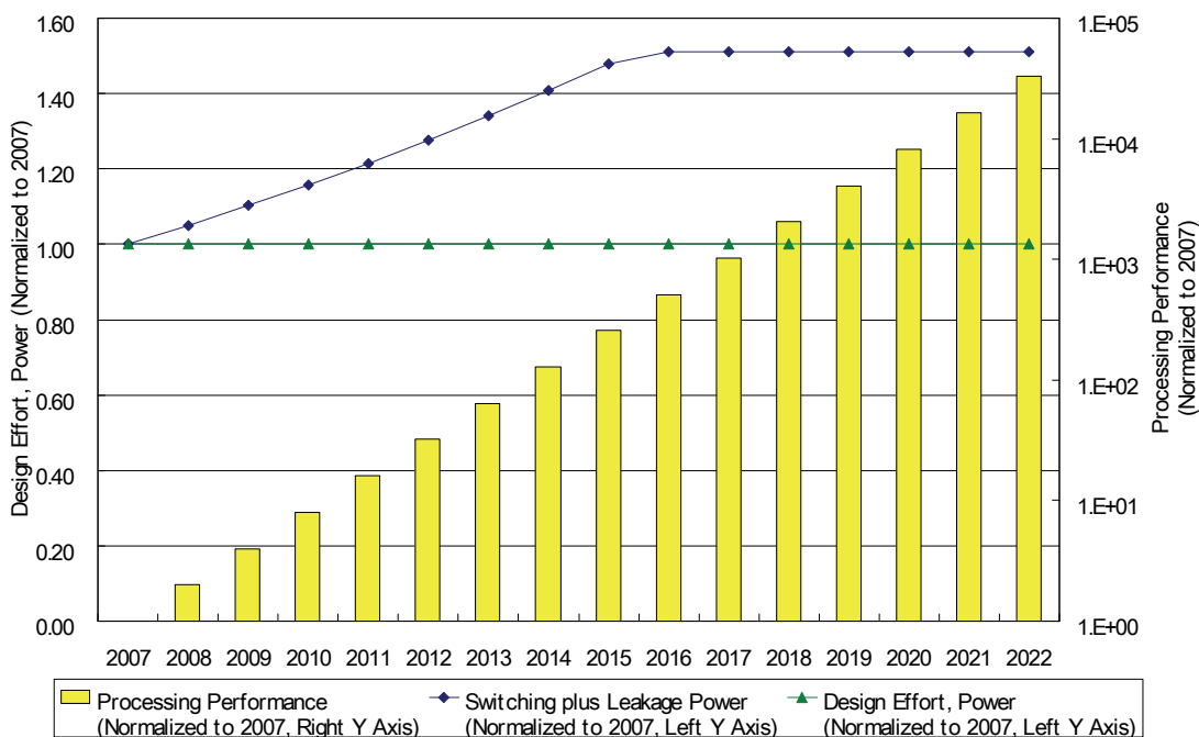
Figure SYSD3 Several Trends for SOC Consumer Portable Driver
