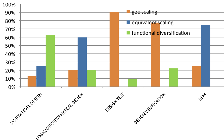
Figure DESN10 Moore and Non-Moore Design Technology Improvements
