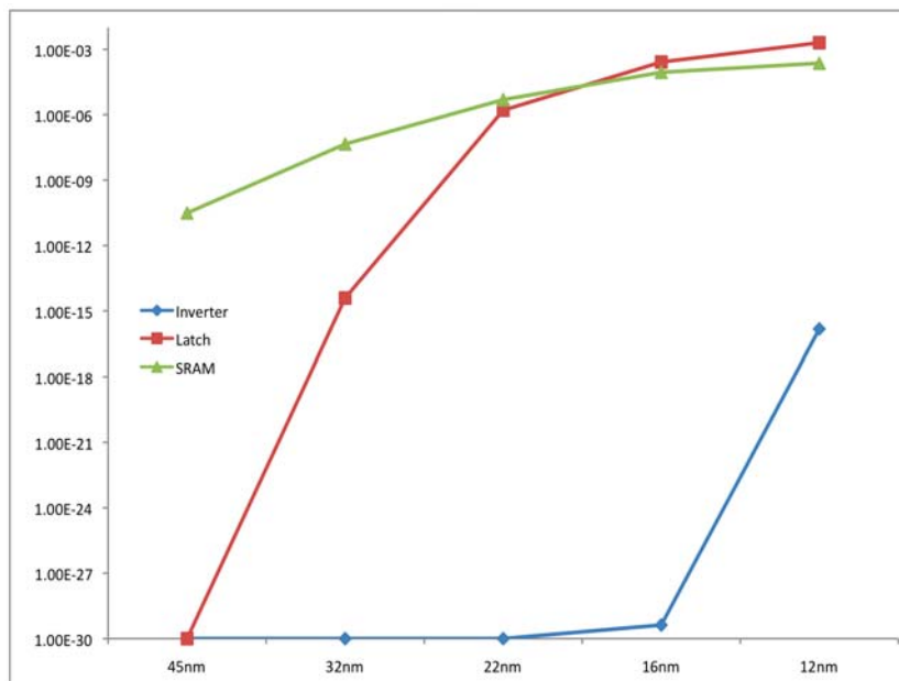
Figure DESN8 Variability-Induced Failure Rates for Three Canonical Circuit Types
