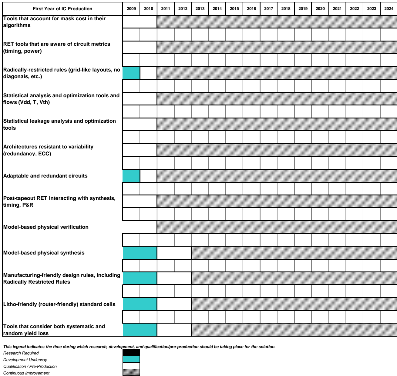
Figure DESN9 Design for Manufacturability Potential Solutions
